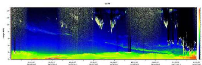
High altitude aerosols descends and merges into local a boundary layer over 3-day period
