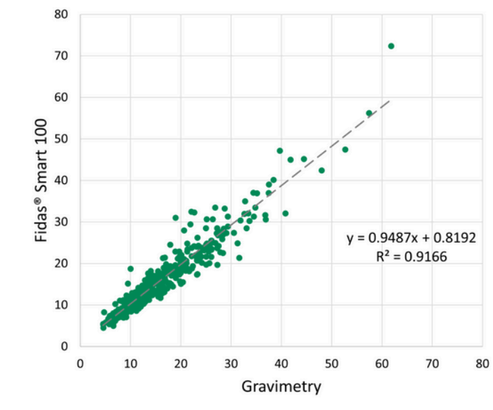
Fig. 2: Fidas® Smart 100 vs. Gravimetry PM 10
